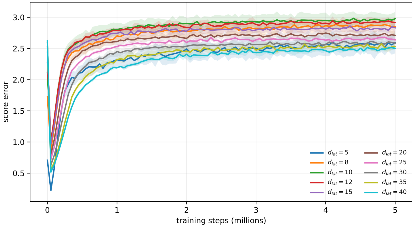
Score error over training, 5-seed mean with 95% CI
